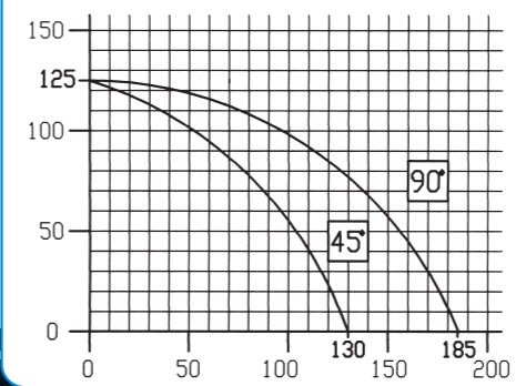
Diagramma di taglio lama Ø 400 Cutting diagram saw blade Ø 400
